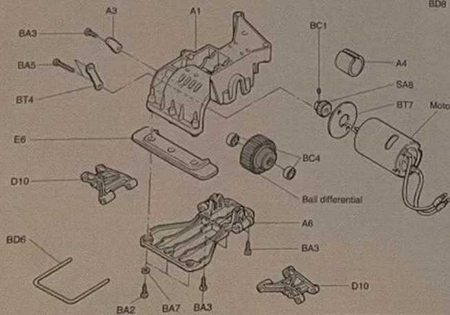
(Gearbox)
