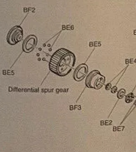
(Ball Differential)
