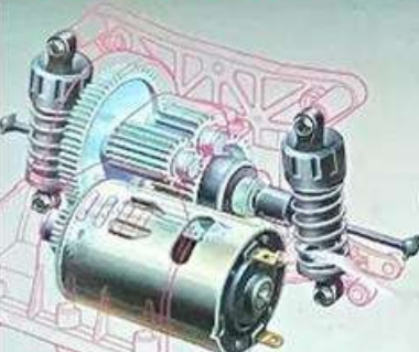
540 TYPE MOTOR
